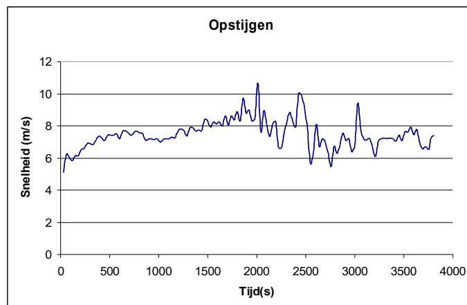
Figure 4: Vertical velocity (m/s) vs time (s) during ascent
