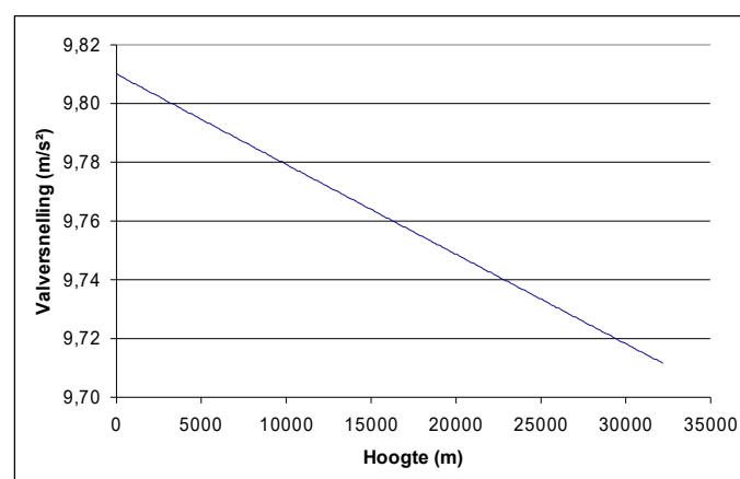
Figure 24: Gravitational acceleration (theoretical values in m/s²) vs altitude (m asl.)
